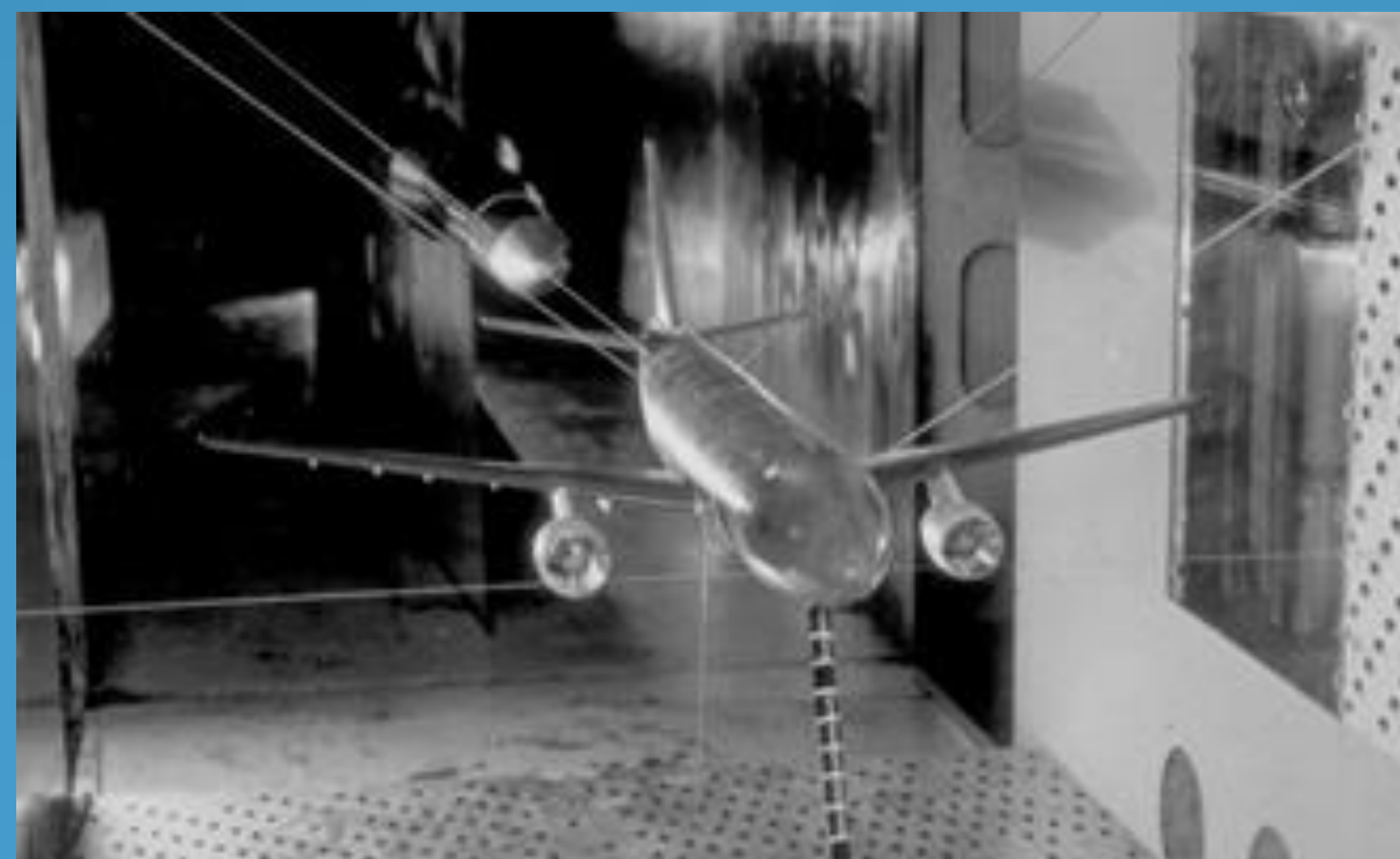
Wind tunnel testing of a scale model [2]
