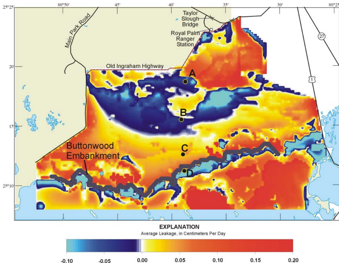
Figure 5. Map showing average leakage rates for the simulation period. Graphs for the four locations are shown in Figures 6, 7, 8, and 9. Positive leakage rates represent downward flow into the aquifer. Negative leakage rates indicate upward flow from the aquifer to the surface water.
