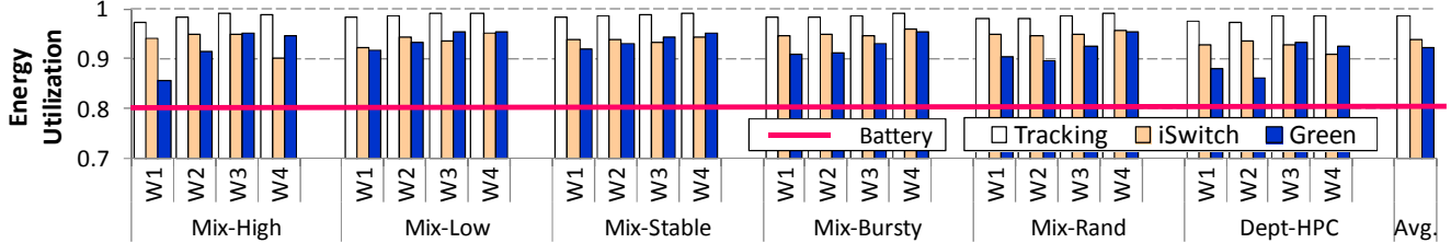
Figure 16: The normalized overall wind energy utilization
